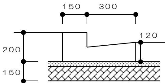
L型側溝
